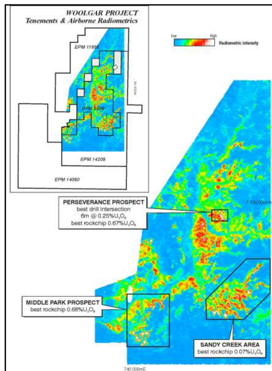
Figure 3. Airborne radiometric data (uranium channel) & uranium prospect locations. Unconformity style uranium mineralisation targets correspond to the white areas on the image.
