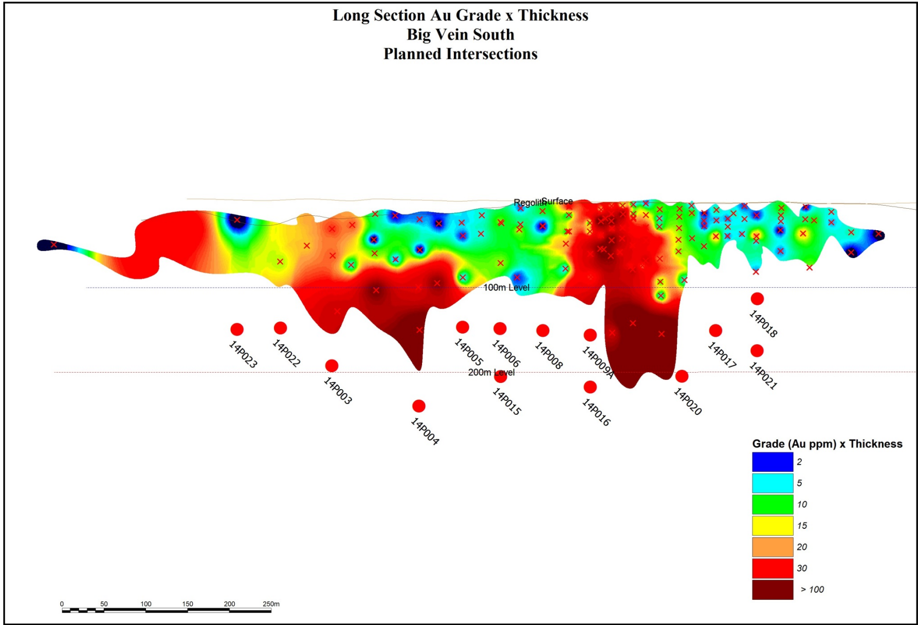
Figure 2: Long Section of BVS showing the gold grade x thickness (g/t x m), previous drill intersections (red crosses) and the proposed drillhole intersections from the current program (red dots)
